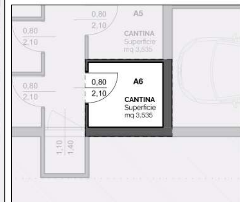
Piano interrato
